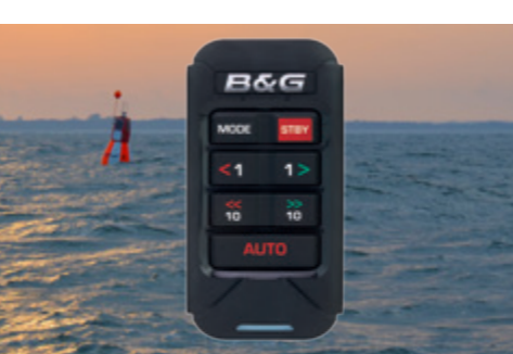
B&G autopilot control unit & fluxgate Gyro Compass RC42
